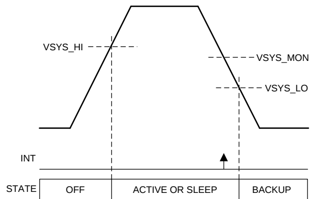
Figure 4. State Transitions
