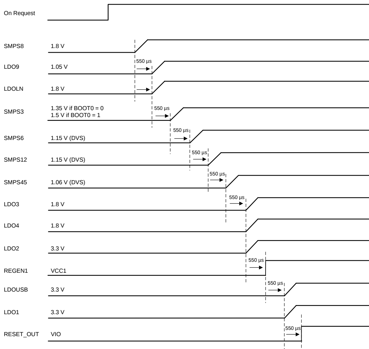
Figure 6. OFF2ACT Sequence of TPS6590376ZWSR
