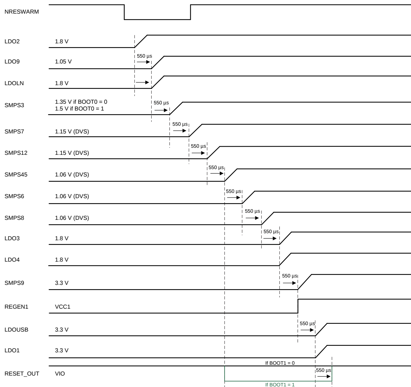
Figure 13. Warm Reset Sequence of TPS6590377ZWSR
